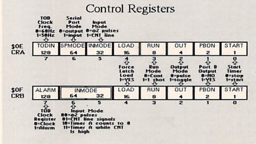
Figure 6. Control registers.
